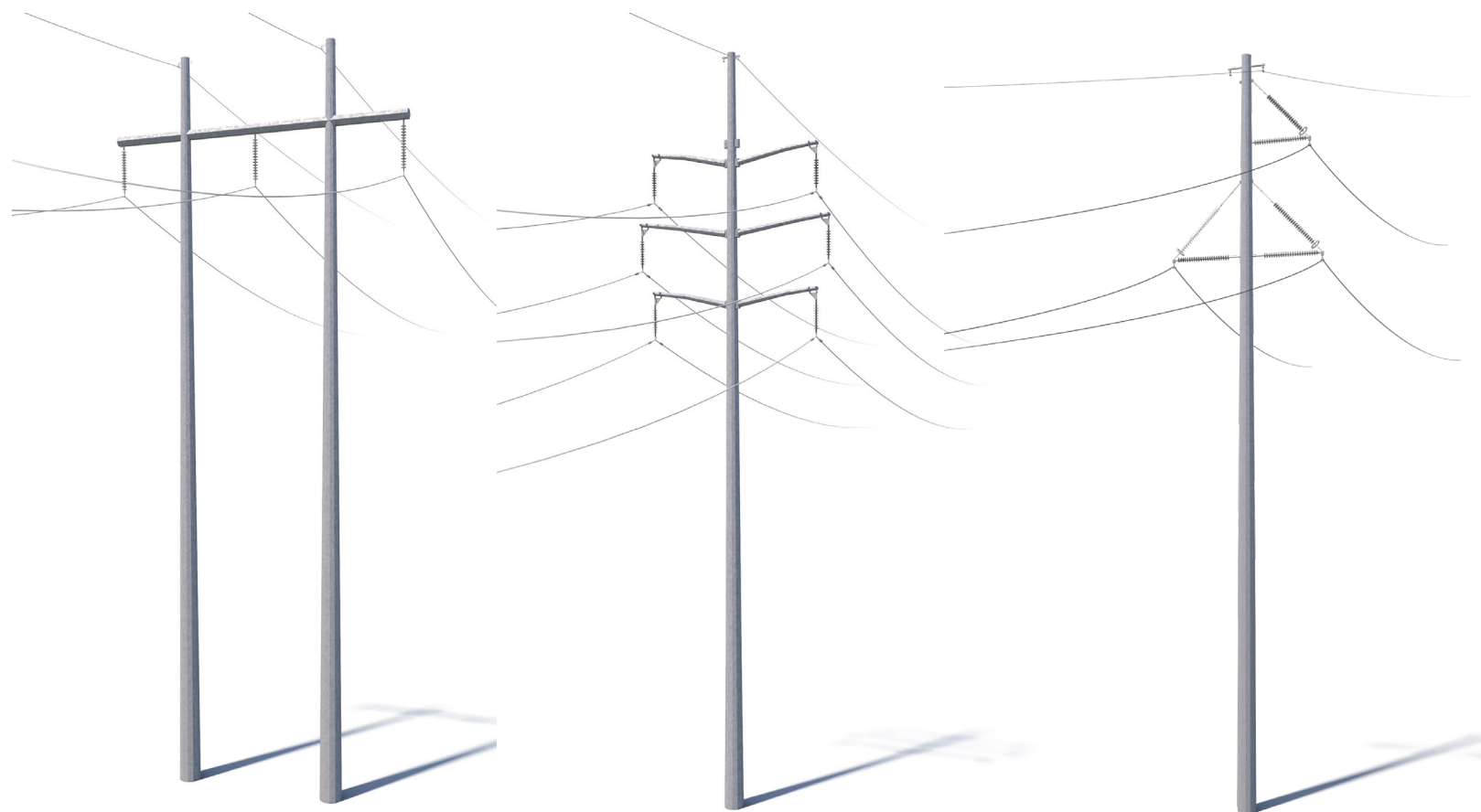
Single Circuit H-Frame
